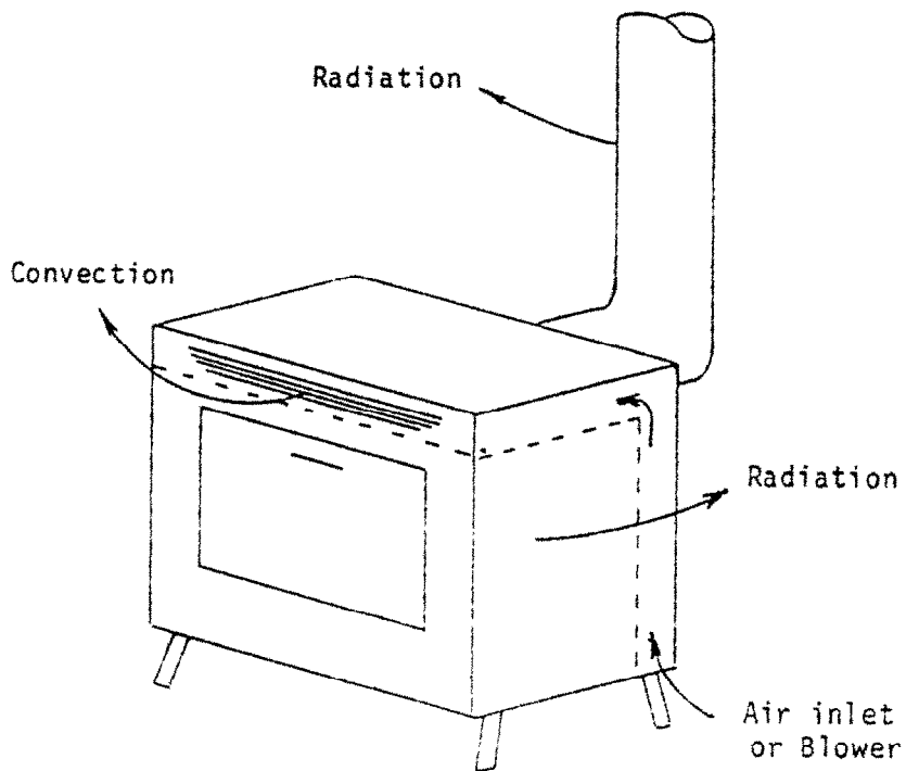
CONVECTION STOVE
